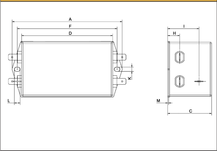
Connection style -1, 8A to 30A types
