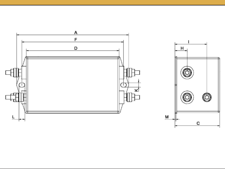
Connection style -6, 10A to 30A types
