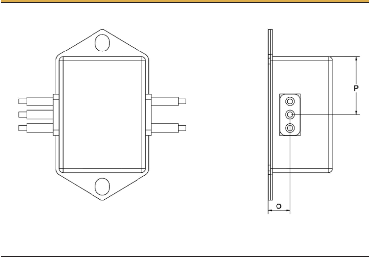
Connection style -3, 1A type
